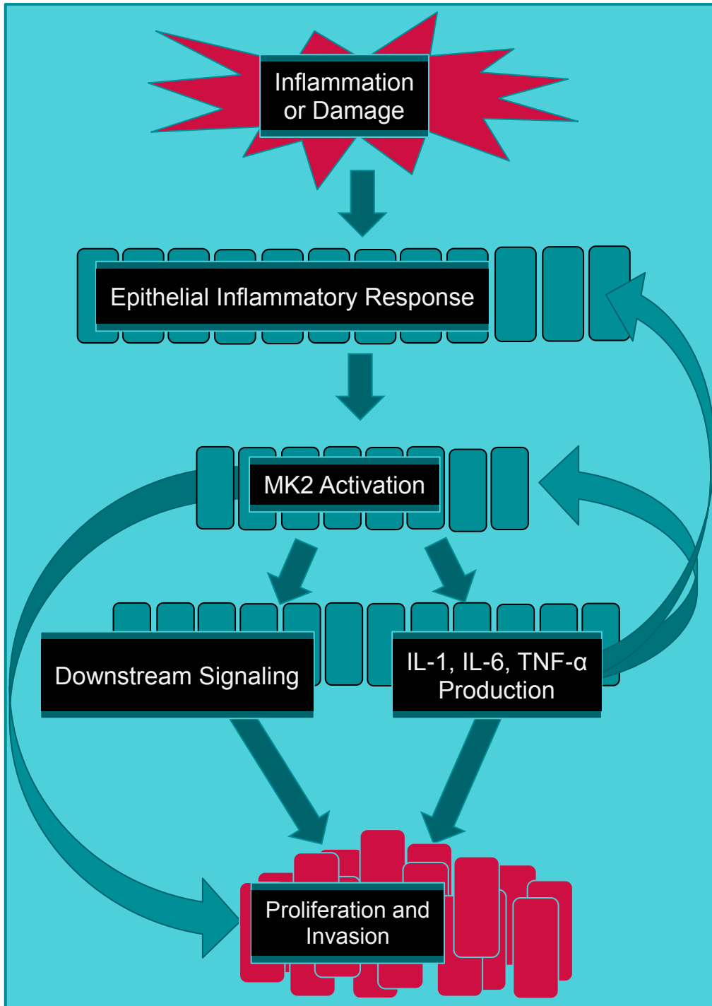
Figure 2. Proposed effects of MK2 signaling during CRC.
